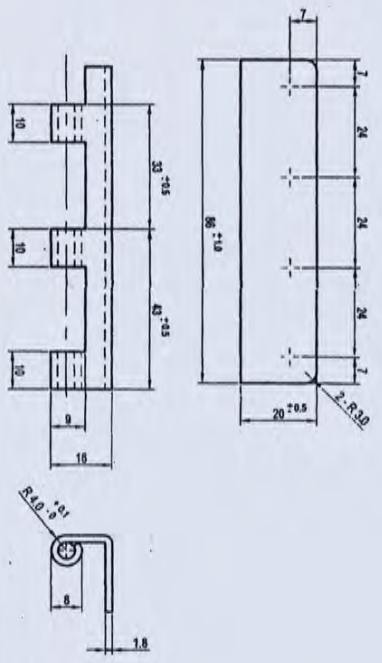
12 COVER HINGE
