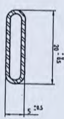
SECTION C - C
